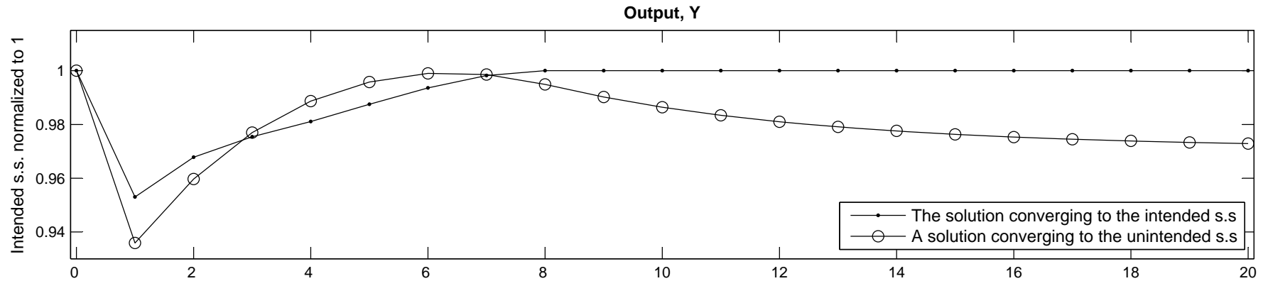
Figure 2: Two solutions of the model in Section 3
